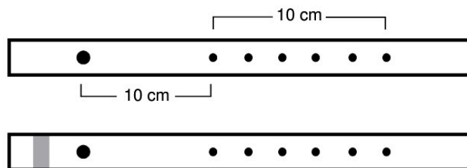
Sketsa suling bambu
